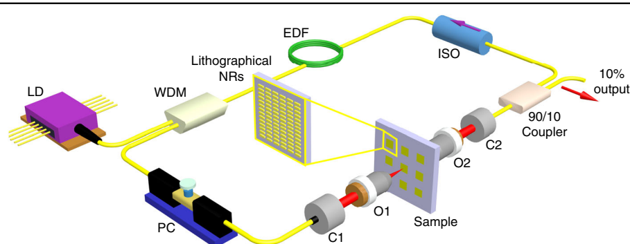
Fig. 4 Scheme of a home-built ultrafast fiber laser that integrates lithographical NRs as a saturable absorber, where LD represents the laser diode, WDM is the wavelength-division multiplexer, EDF is the erbium-doped fiber, ISO is the optical isolator, PC is the polarization controller, C1 and C2 are the collimators, and O1 and O2 are the objectives
